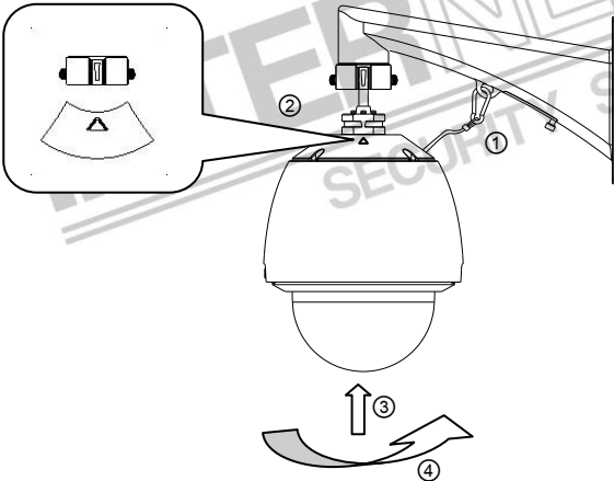
Figure 2-6 Align the Labels
