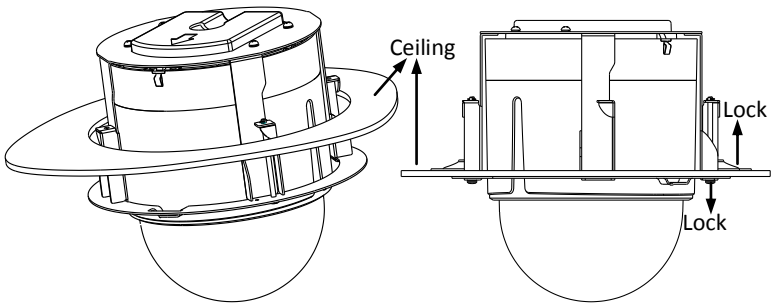
Figure 2-11 Install the back box
