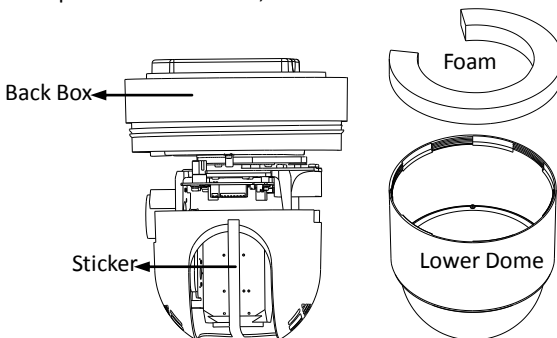
Figure 2-14 Remove the Protective Accessory
