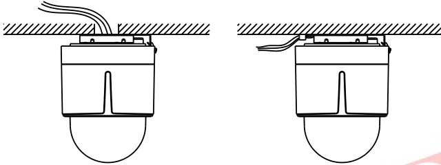
Figure 2-13 Cabling for Ceiling Mounting
