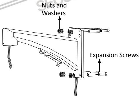
Figure 2-4 Install the Wall Mount
