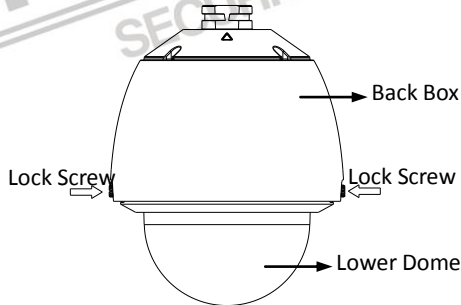
Figure 2-2 Disassemble the Speed Dome
