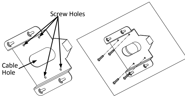
Figure 2-15 Mark the Screw Positions
