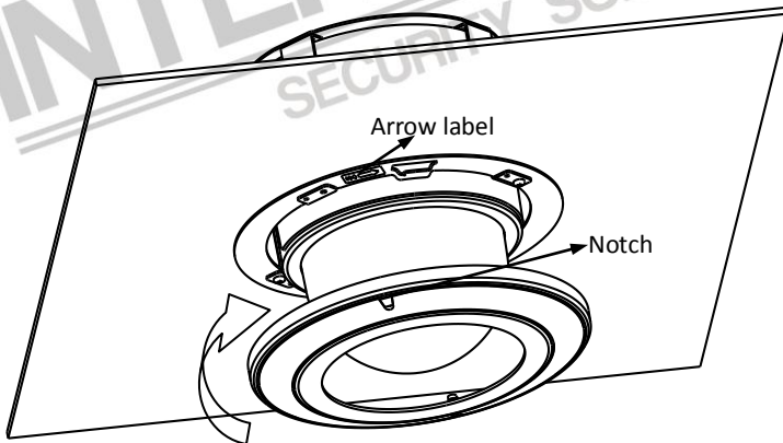
Figure 2-12 Install the Trim Ring
