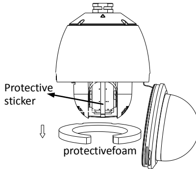
Figure 2-3 Disassemble the Speed Dome
