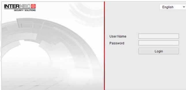
Figure 4-1 Login Interface
