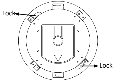
Figure 2-9 Locks and Lock Screws
